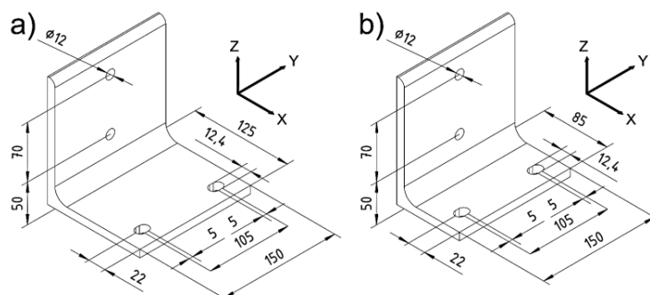
Figure 33 – Supports muraux – version: a) version standard, b) version raccourcie
