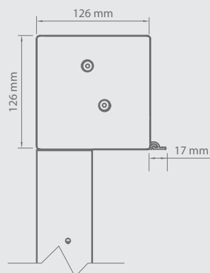
Cassette dimensions
