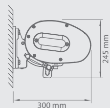
Wall installation
