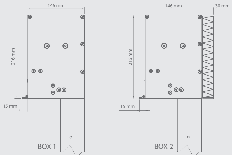
Cassette dimensions
