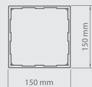
Post cross-section
