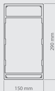
Beam cross-section
