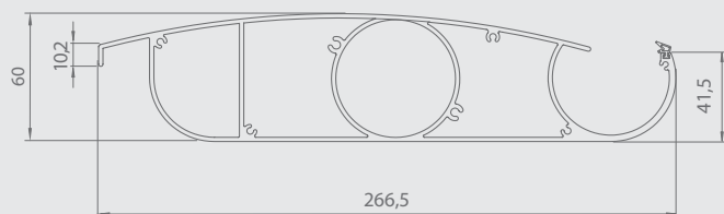
Post cross-section
