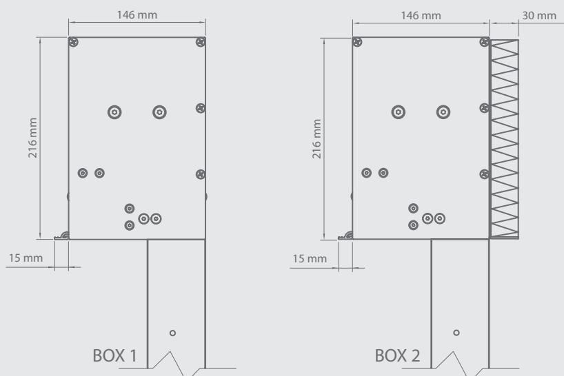
Cassette dimensions
